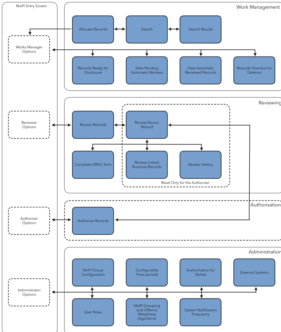
Figure 2 MoPI Manager Screen Flow
