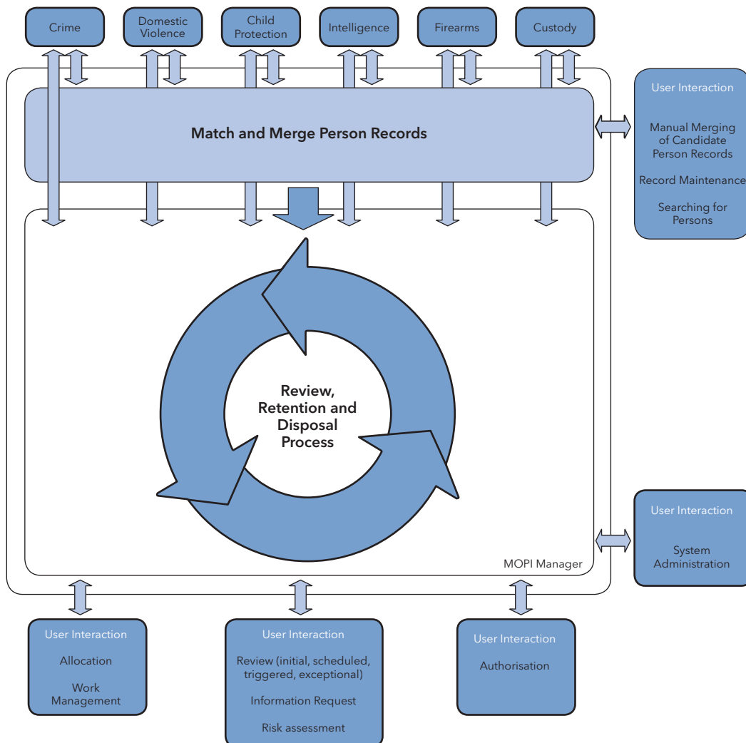
Figure 1 - System Context
